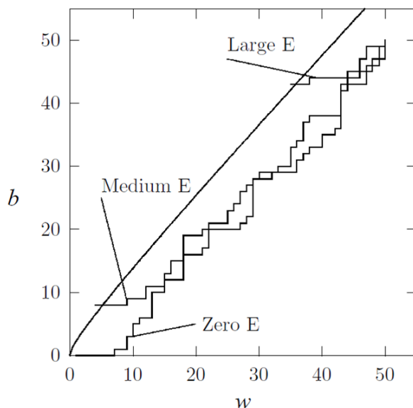
Figure 5: Three different realisations of the game with the optimal strategy (the smooth curve is the threshold boundary where play is stopped)
