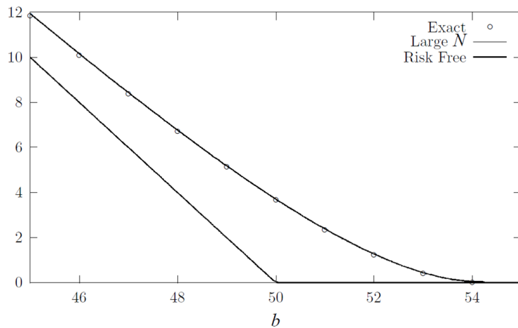
Figure 1: The value as a function of b for an N = 100 hat
