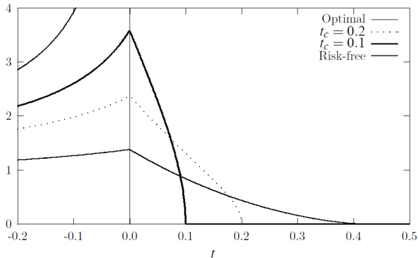
Figure 3: The Sharpe Ratio as a function of t for a variety of strategies
