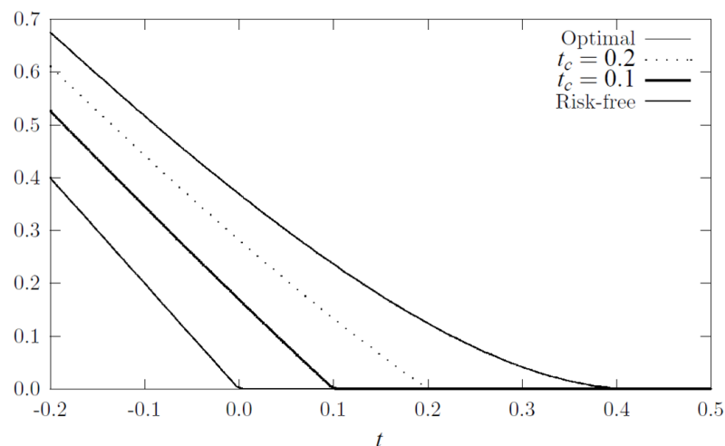
Figure 2: f(t) for a variety of strategies
