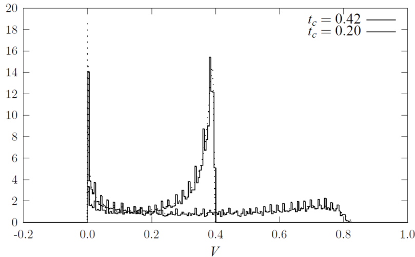
Figure 4: The probability distribution of the scaled value V for t = 0 and two choices of strategy, the optimal strategy and the t_c = 0.20 strategy
